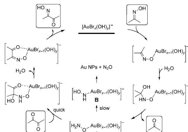
Scheme 3. Plausible mechanism for the hydrolysis of acetone oxime in the presence of gold(III) and diacetyl at neutral pH.
